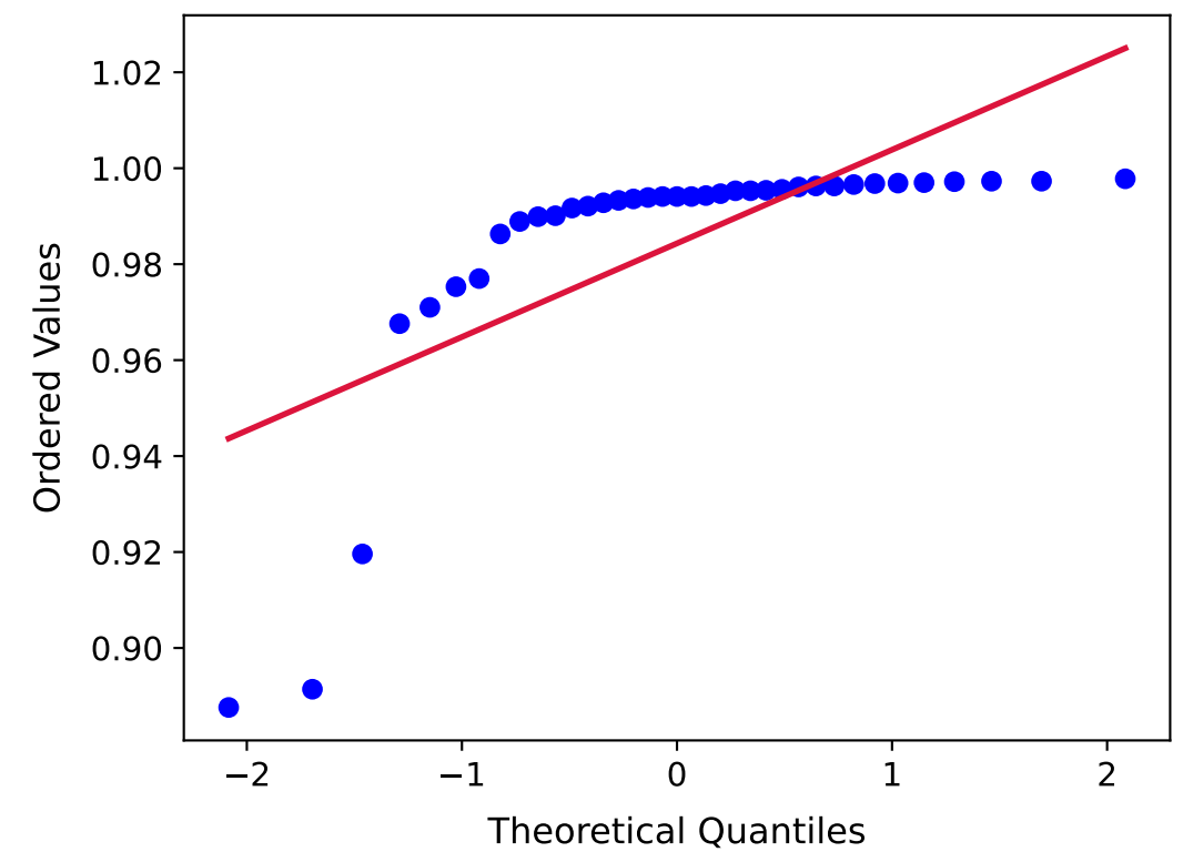
Hybrid Q-Q Plot
