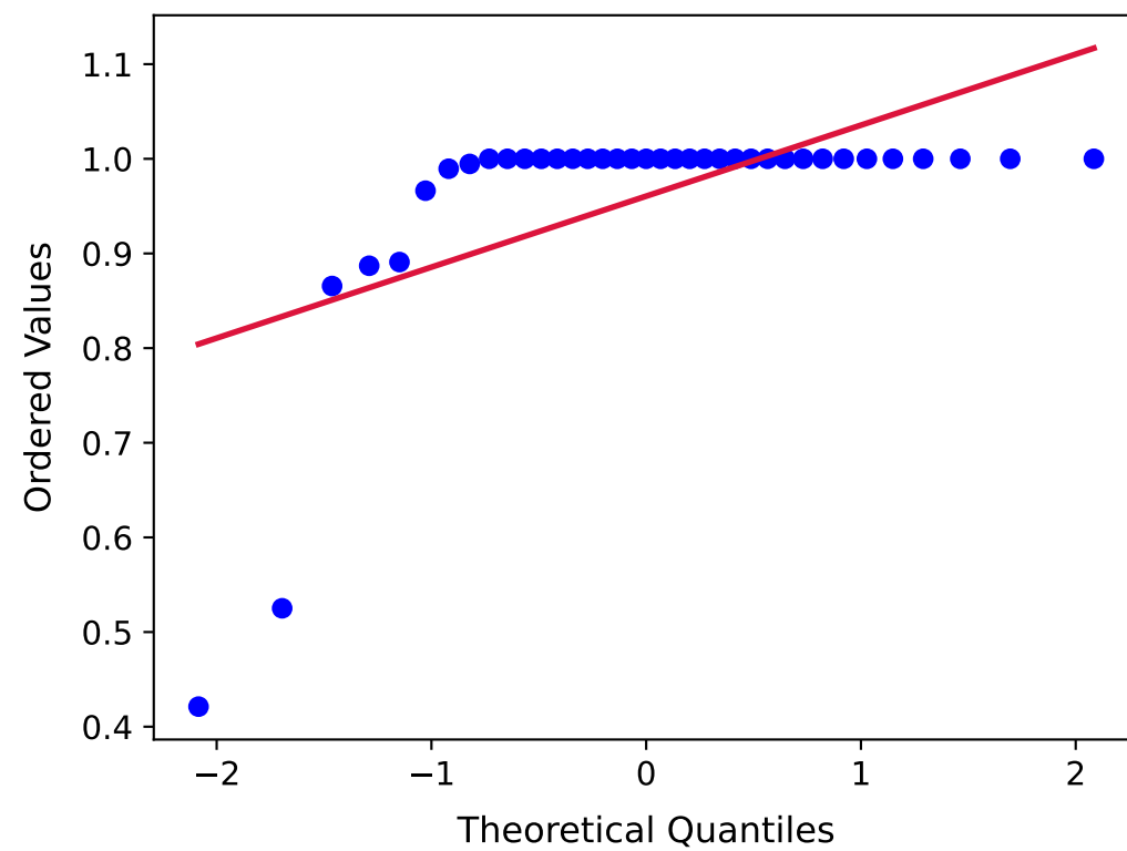
SAM2 Q-Q Plot
