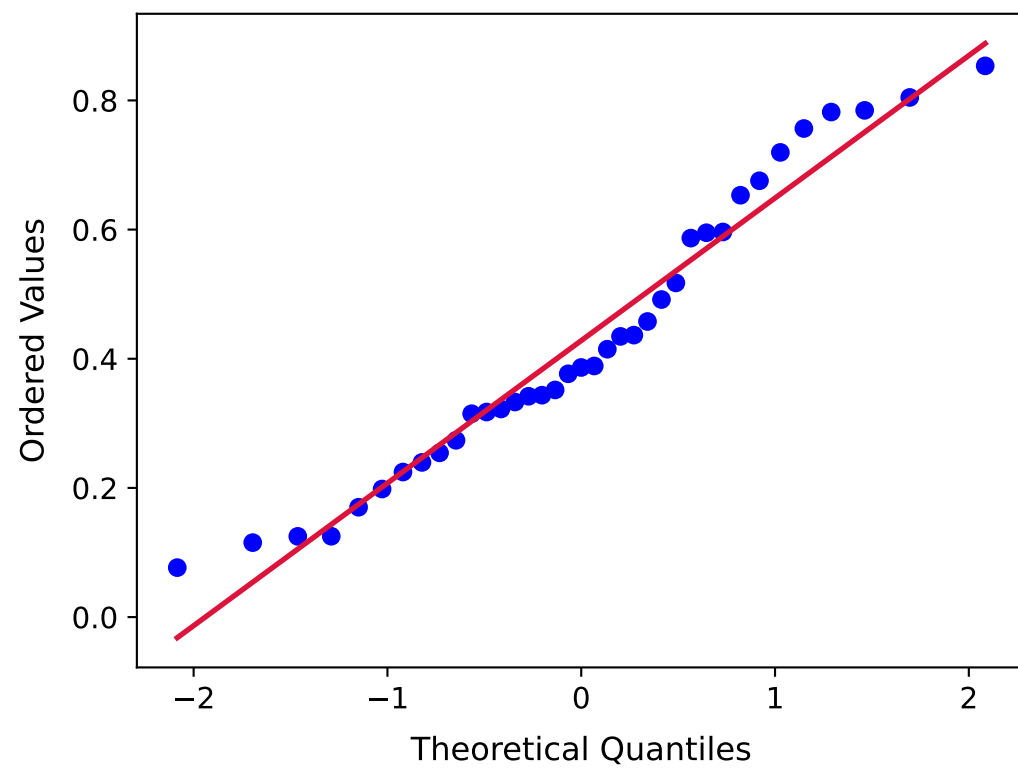
Mahalanobis Q-Q Plot
